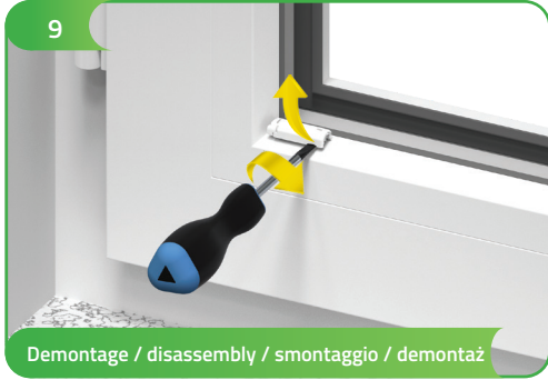
Demontage / disassembly / smontaggio / demontaž
